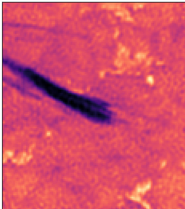
Fitted @ 6561.278 Å (idx=1)
