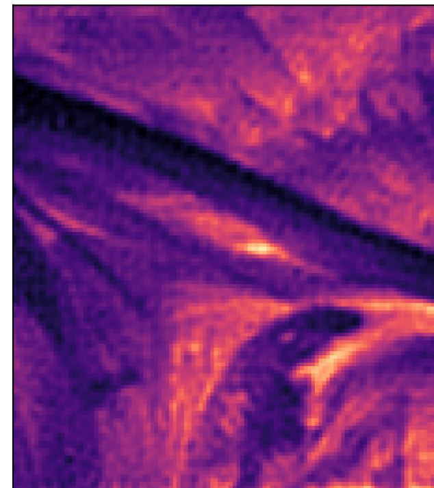
Fitted @ 6562.809 Å (idx=181)
