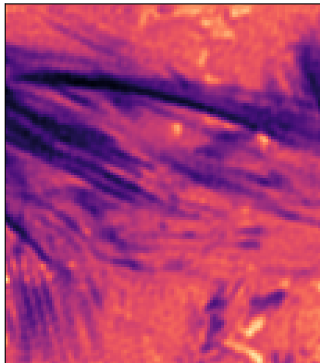
Fitted @ 6562.043 Å (idx=91)
