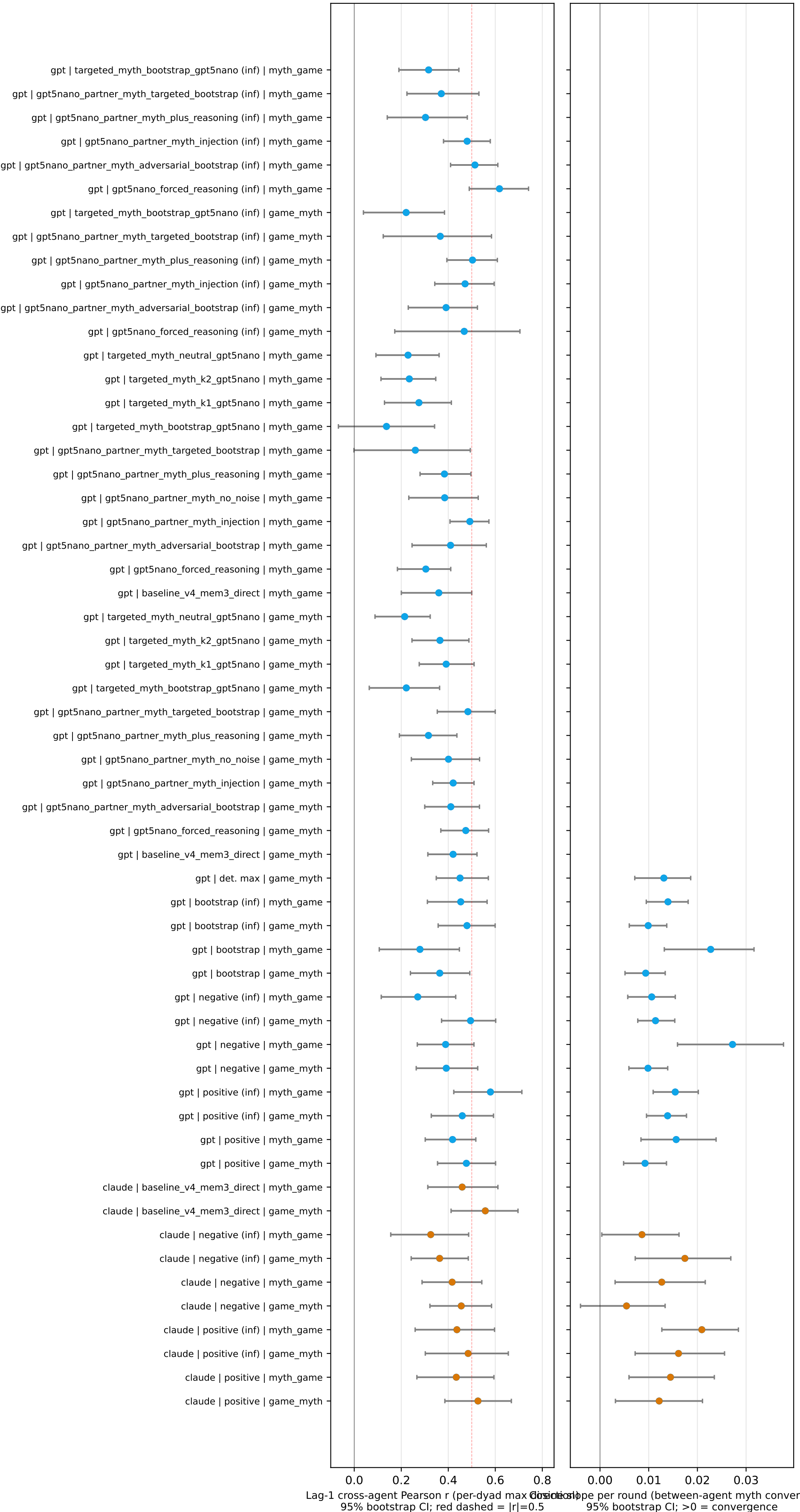
(a) Cooperativity-language lag-1 correlation (b) Embedding-cosine convergence slope
