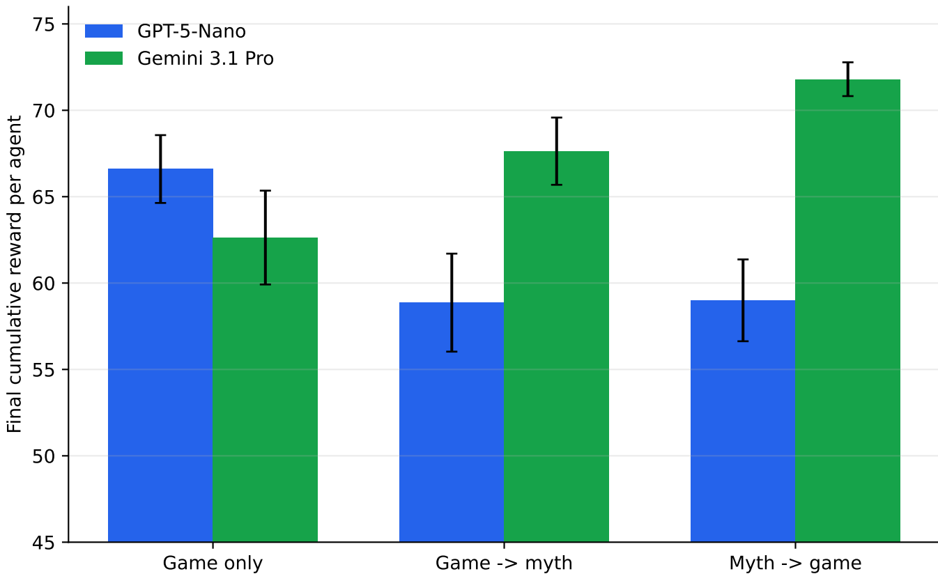
Bootstrap standard prompt: GPT-5-Nano destabilises, Gemini does not
