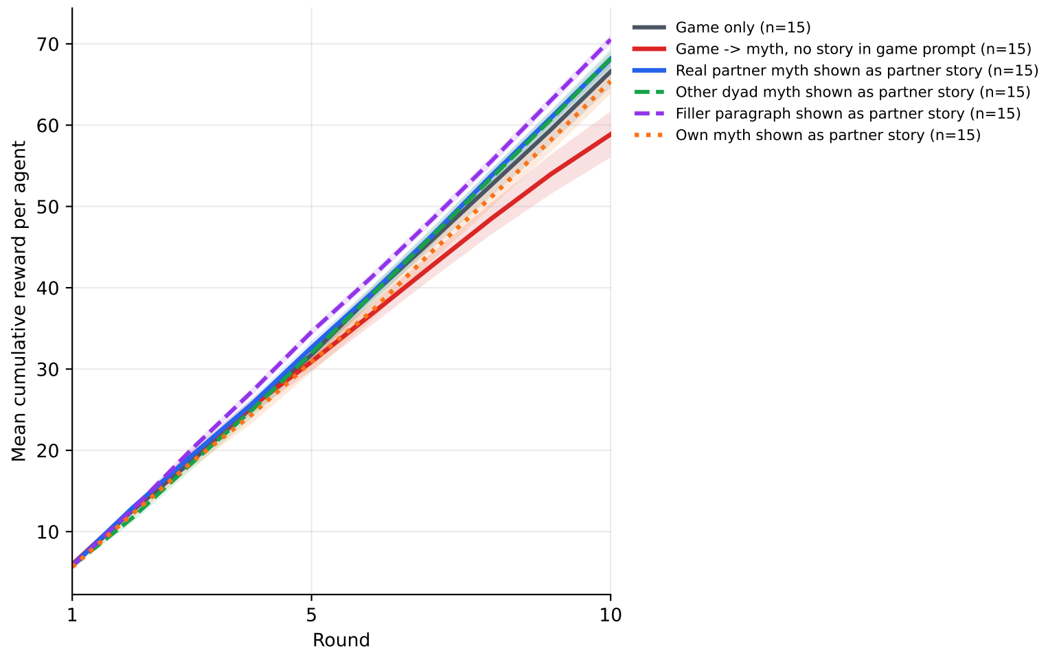
GPT-5-Nano bootstrap: text labelled as partner story restores cooperation
