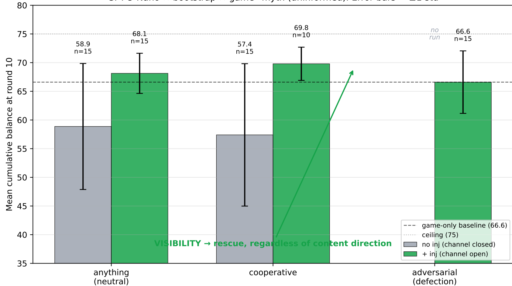
Bootstrap-noise rescue: 2×3 factorial of visibility × content GPT-5-Nano × bootstrap × game→myth (uninformed). Error bars = \pm 1 std
