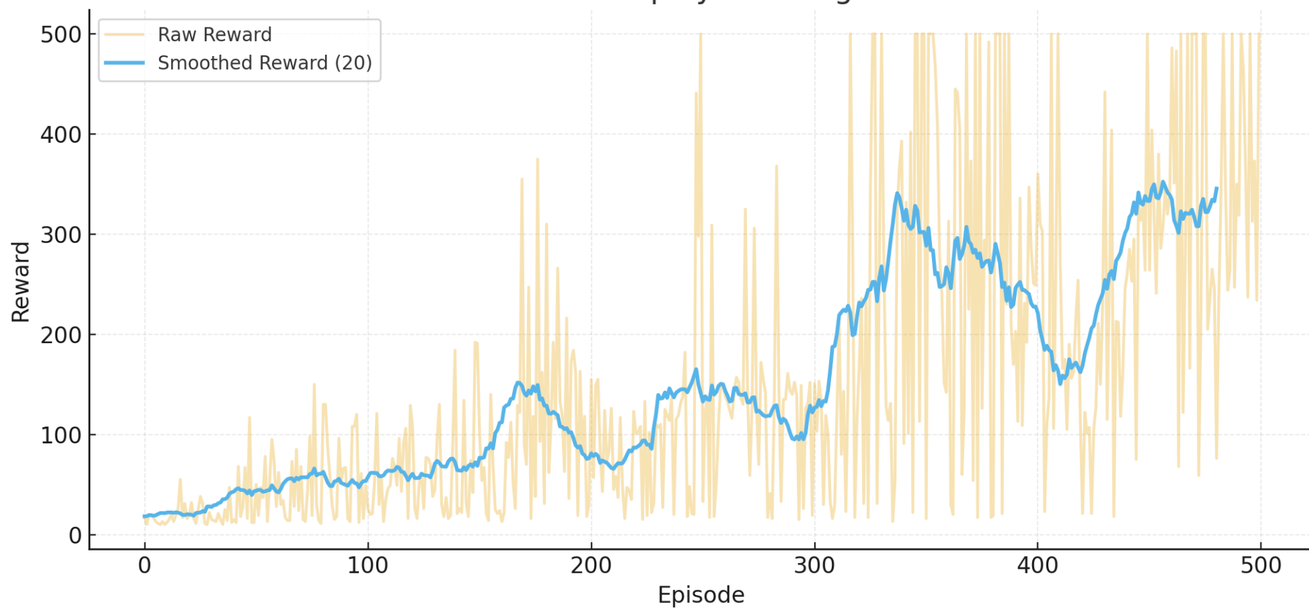
Prioritized Replay Learning Curve
