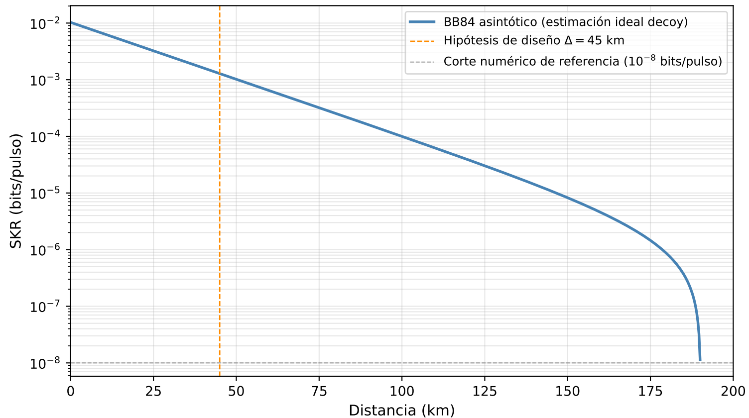
Tasa de clave secreta BB84: modelo asintótico ideal ( \alpha = 0.2 dB/km, \eta = 0.1 , \mu = 0.5 , e_{det} = 0.015 , q = 1/2 )
