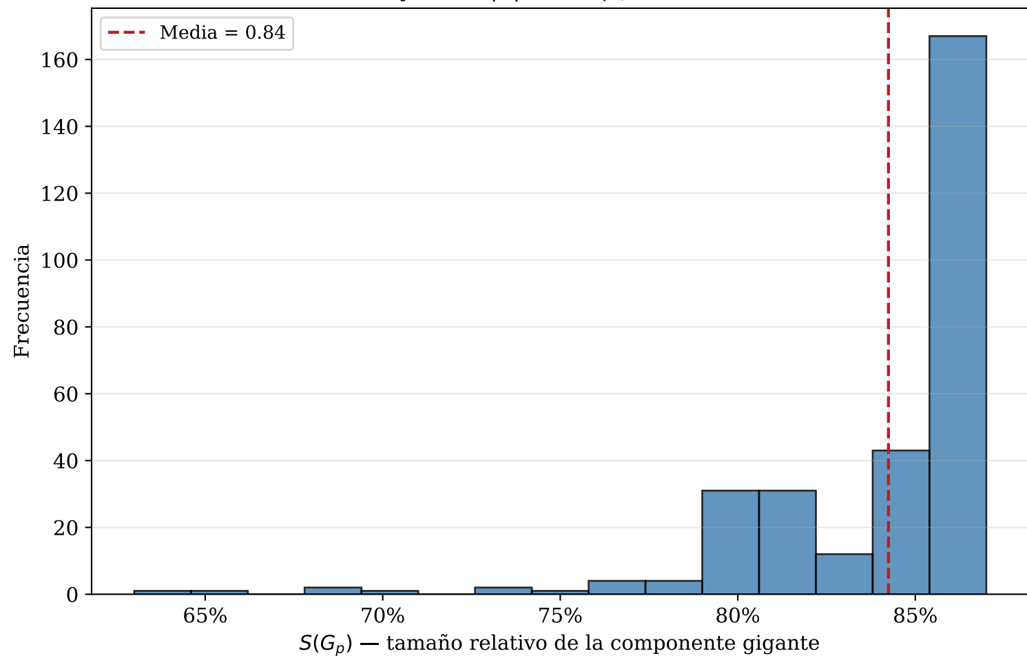
Castilla y León ( |V| = 100 , p_0 = 13\% , R = 300 )
