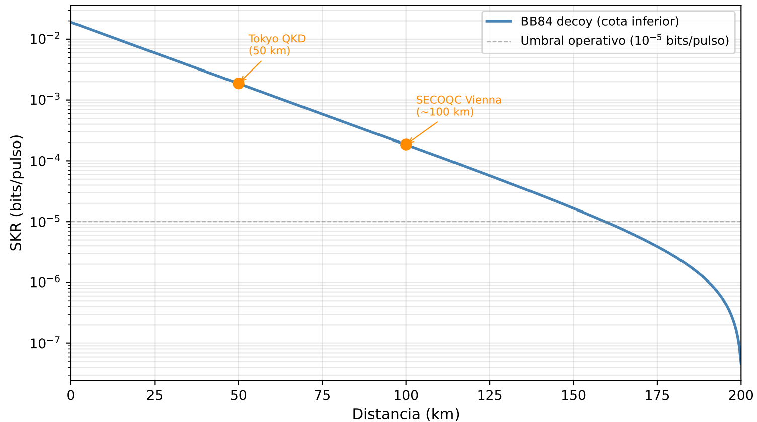
Tasa de clave secreta BB84 con decoy states ( \alpha = 0.2 dB/km, \eta = 0.1 , \mu = 0.5 , e_{det} = 0.015 )
