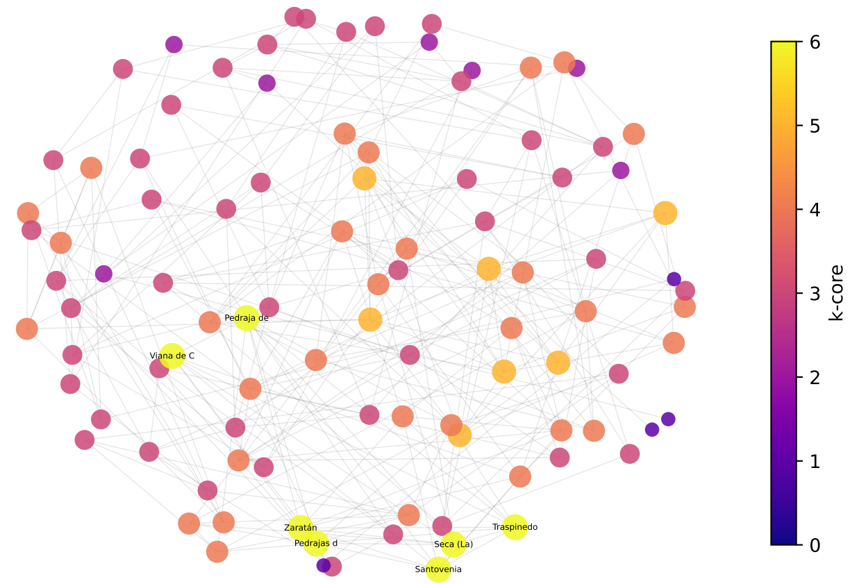
CyL ( |V|=100 ) k_{max} = 6 , inner core: 7 nodes
