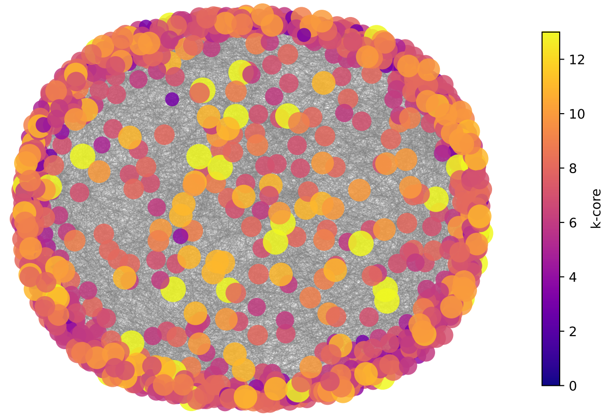
Spain ( |V|=950 ) k_{max} = 13 , inner core: 35 nodes
