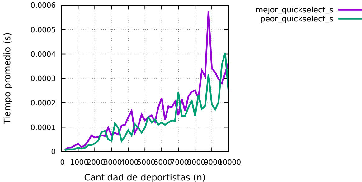
Selection benchmark
