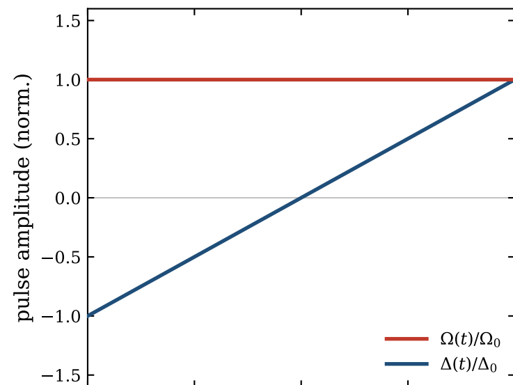
(c) constant-Rabi LMSZ P_1
