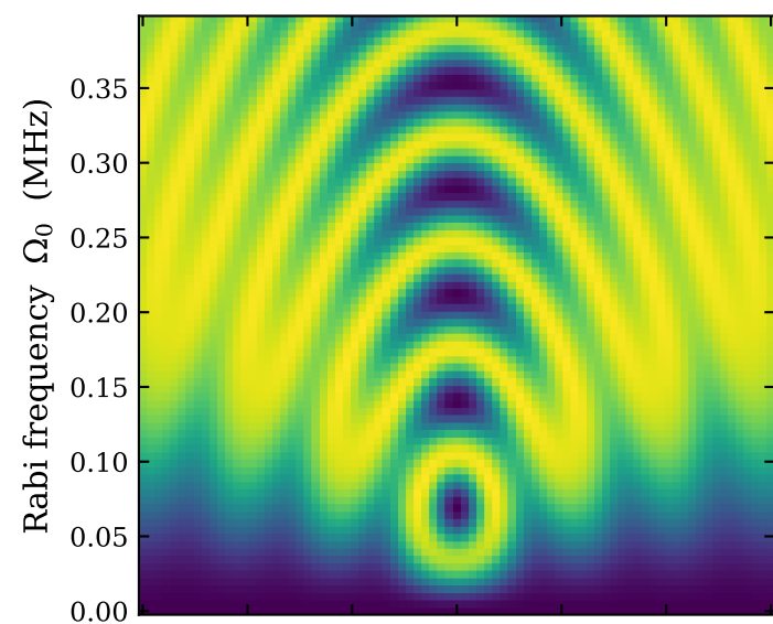
(e) constant-Rabi LMSZ leakage
