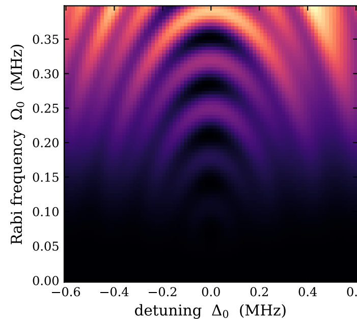
(e) constant-Rabi LMSZ leakage
