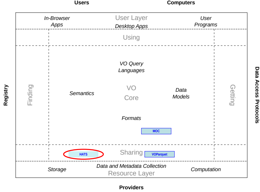
Figure 14: Architecture diagram for this document
