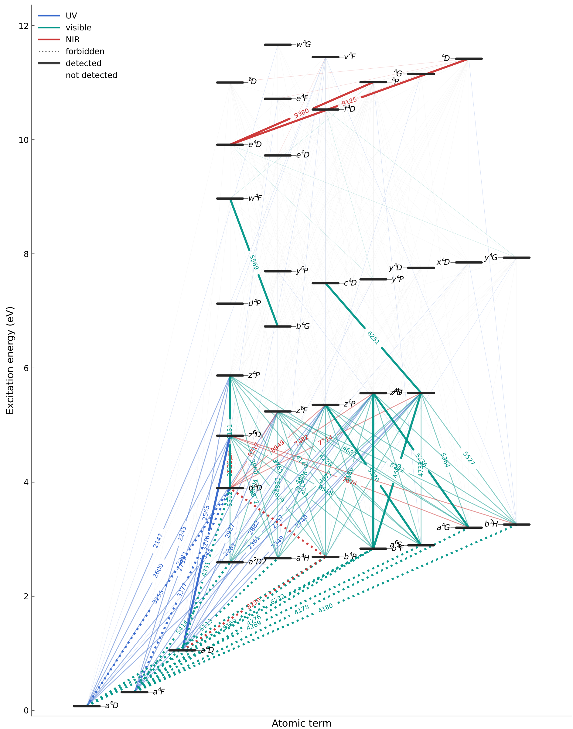
Fe II Grotrian Diagram
