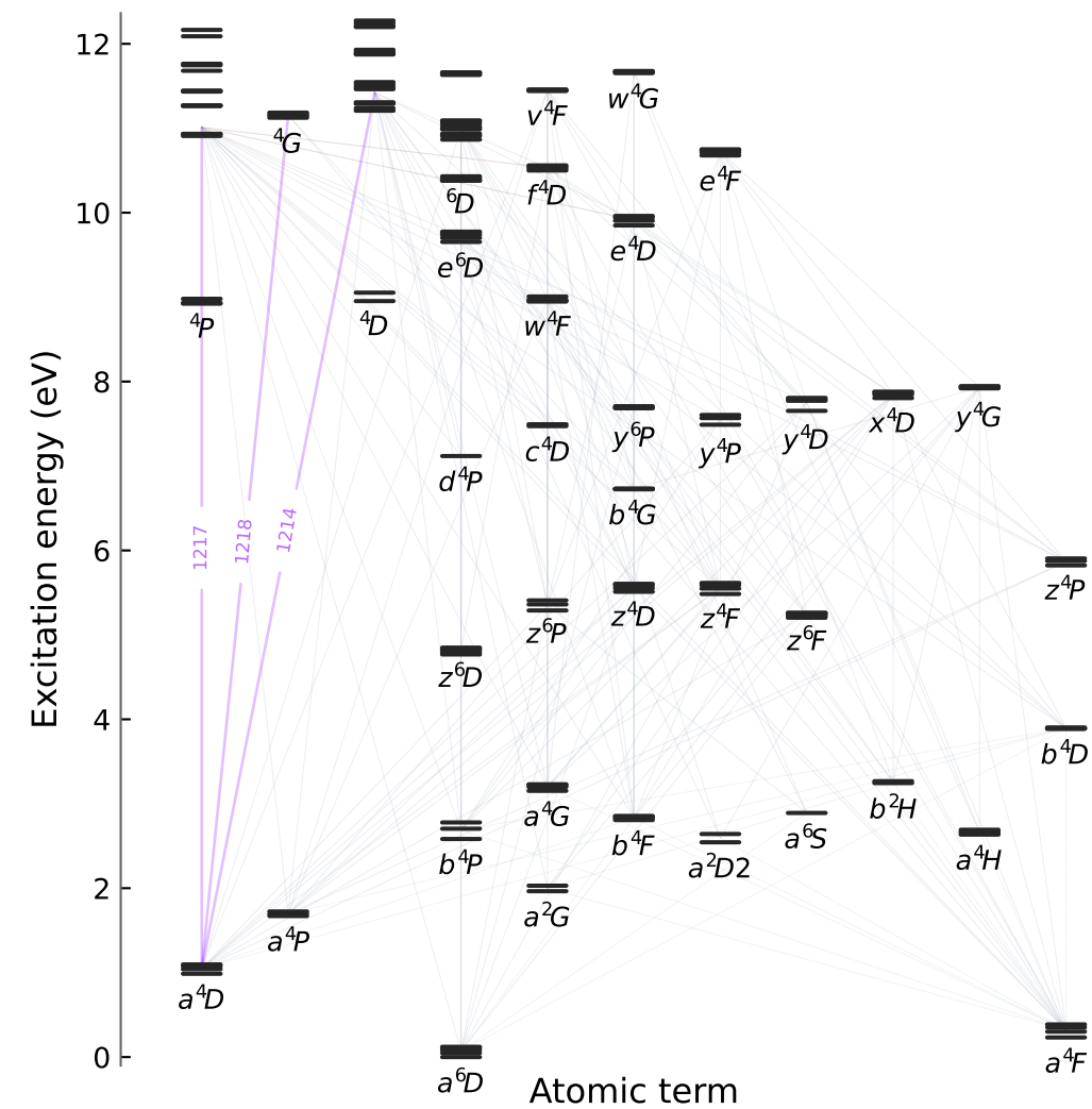
Ly \alpha pumping: a4D \rightarrow 11-12 eV (1216 \pm 3 Å)
