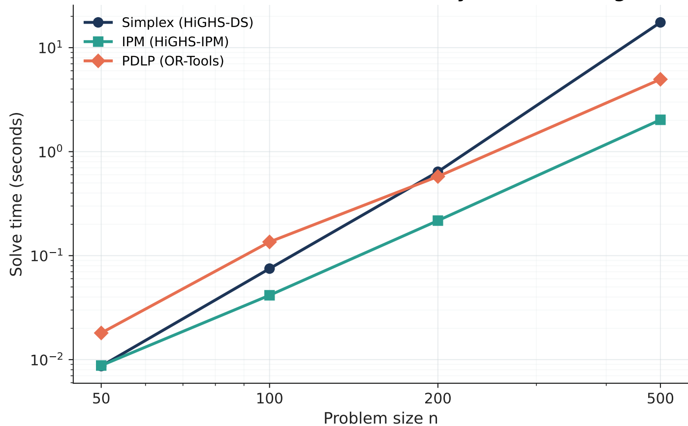
Part 1(a): Exact OT LP Runtime by Solver Paradigm
