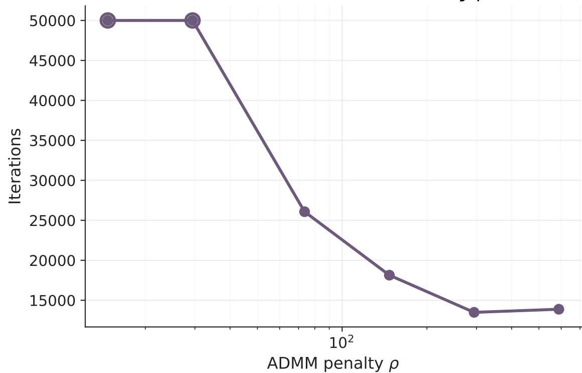
Iterations vs ADMM Penalty \rho
