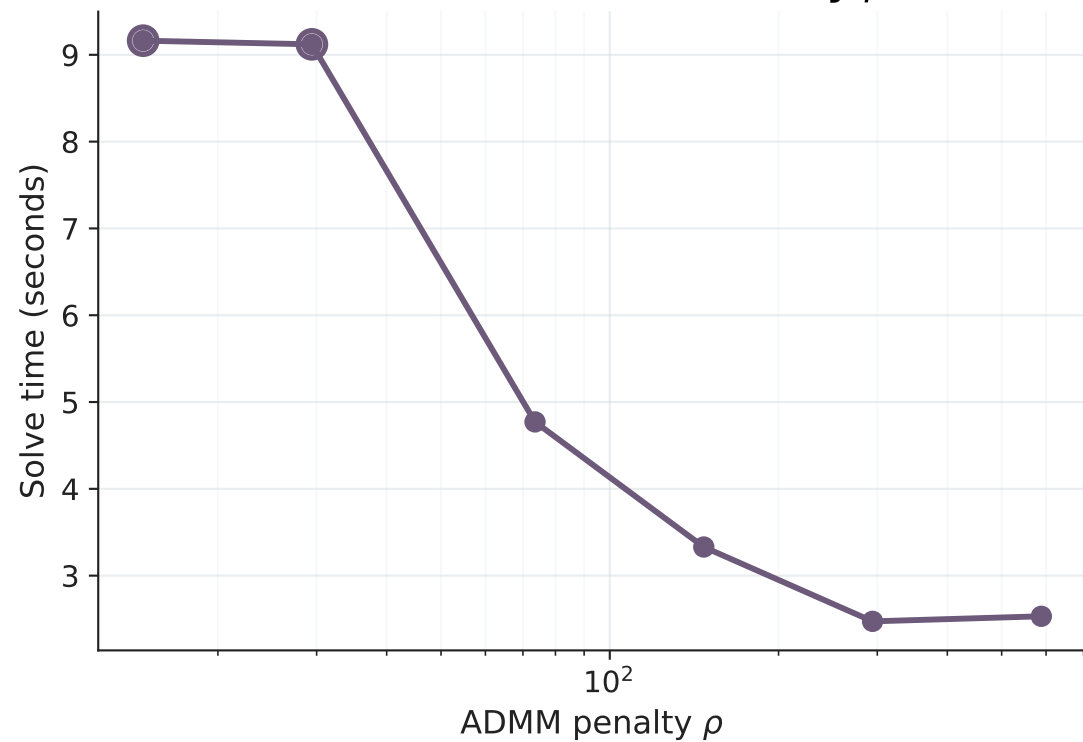
Runtime vs ADMM Penalty \rho
