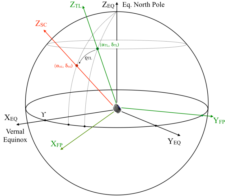
Figure 3: Definition of the Focal Plane reference frame ( X_{FP}, Y_{FP}, Z_{FP} ). The focal plane is defined by the plane ( X_{FP}, Y_{FP} ), where the axis Y_{FP} is in the equatorial plane. Z_{FP} is the optical axis of the telescope, pointing towards the field-of-view.
