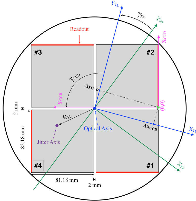
Figure 6: A schematic overview of the focal plane with 4 CCDs. The optical axis Z_{FP} is the blue dot in the middle of the 4 CCDs and points in the positive direction towards the reader. The jitter roll axis Z_{SC} is the purple dot, and also points in the positive direction towards the reader. \gamma_{CCD} is the CCD orientation angle.
