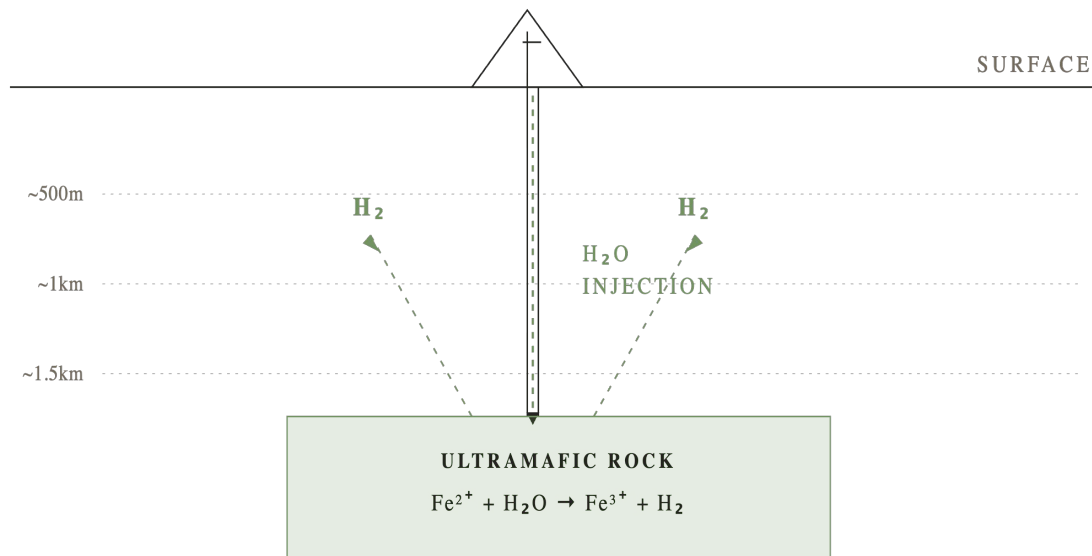
CROSS-SECTION · SERPENTINIZATION REACTION SCHEMATIC
