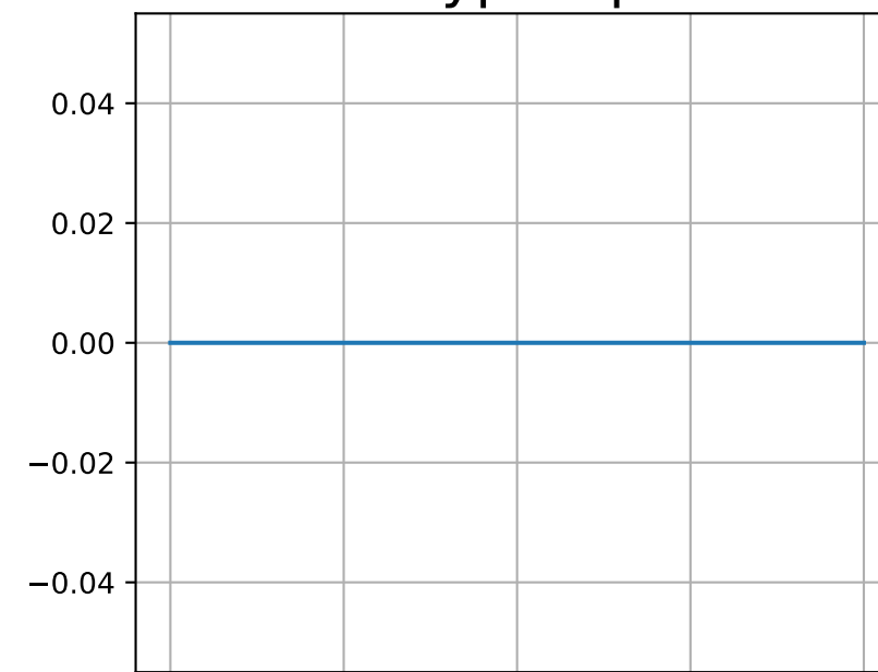
TrainHyperSphere
