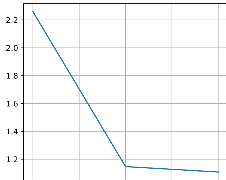
TrainTotal
