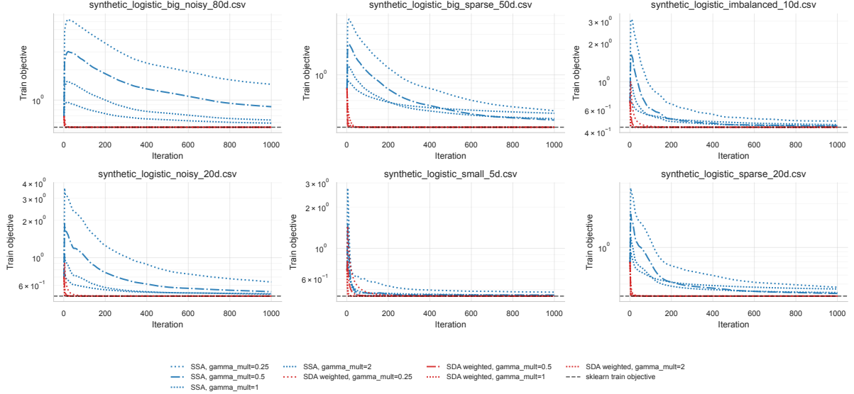
Figure 19: Absolute train objective values for WDA and SSA, with matched sklearn SAGA references.
