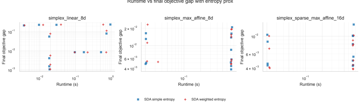
Figure 11: Runtime versus final true objective gap for entropy-prox simplex runs.
