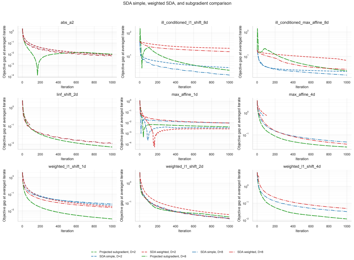
Figure 6: Default comparison of SDA, WDA, and projected subgradient descent on nonsmooth benchmark objectives.
