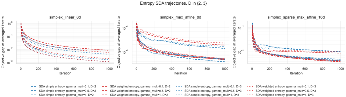
Figure 10: Entropy SDA and entropy WDA on simplex-constrained objectives.
