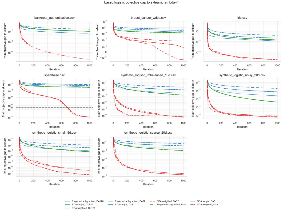
Figure 12: Effect of D on lasso logistic train-objective gap to the sklearn SAGA reference, with \gamma_{\text{mult}} = 1 for SDA/WDA and \alpha = 1 for projected subgradient.
