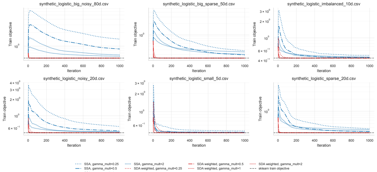
Weighted SDA vs SSA train objective, \lambda=1 , D=128
