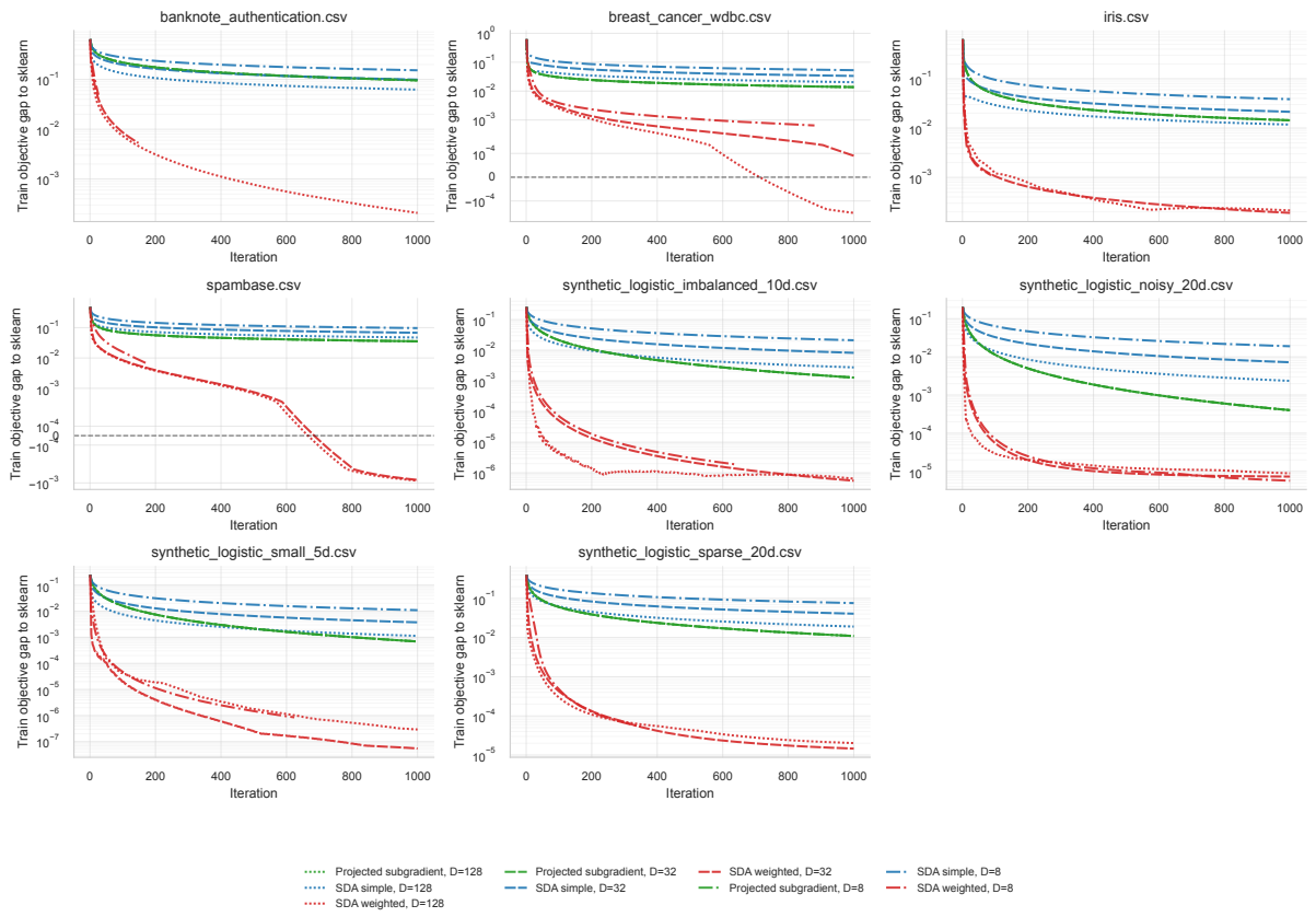
Figure 12: Effect of D on lasso logistic train-objective gap to the sklearn SAGA reference.
