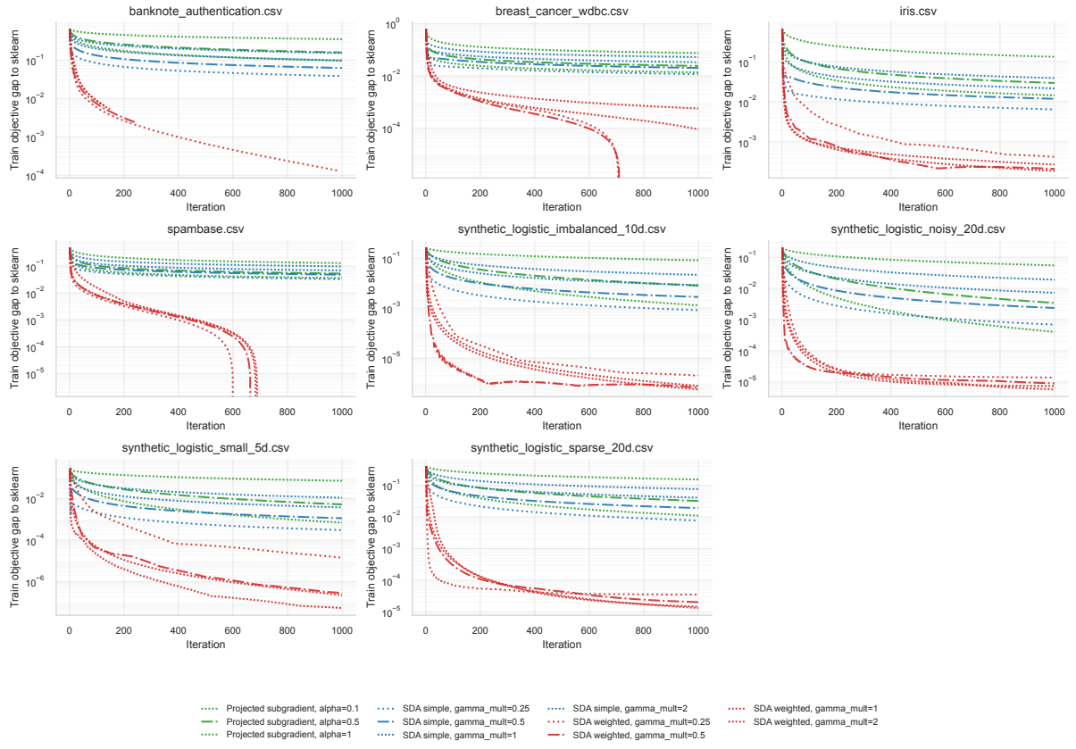
Figure 13: Step-parameter sweep for lasso logistic train-objective gaps at D = 32 .
