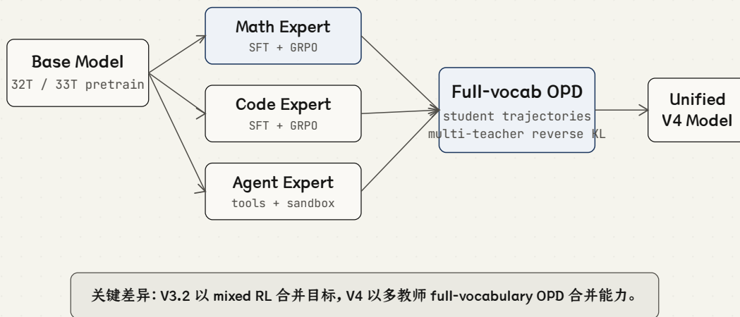
FIGURE 5 post-training pipeline
