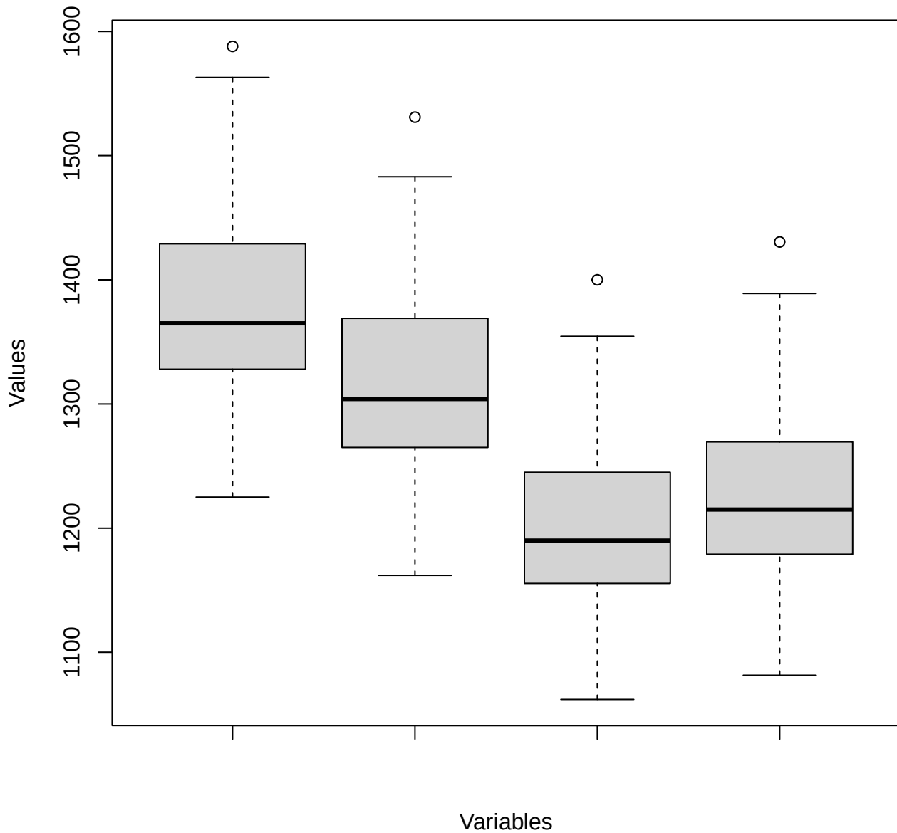
Vertical Boxplots
