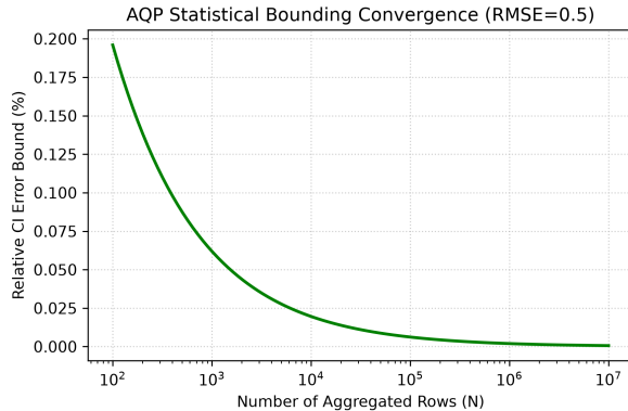
Fig. 2: Theoretical AQP Convergence ( 1/\sqrt{N} ). As the number of aggregated rows N increases, the relative error bound logically shrinks, assuming strictly i.i.d unbiased errors.
