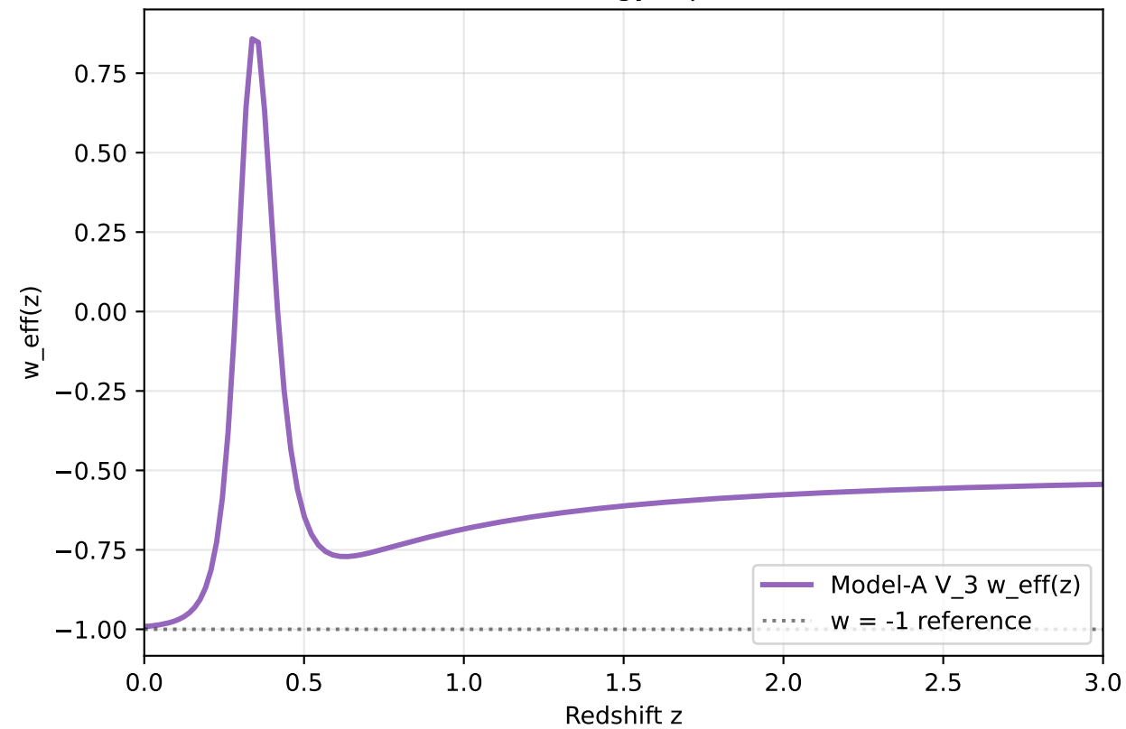
Effective dark-energy equation of state
