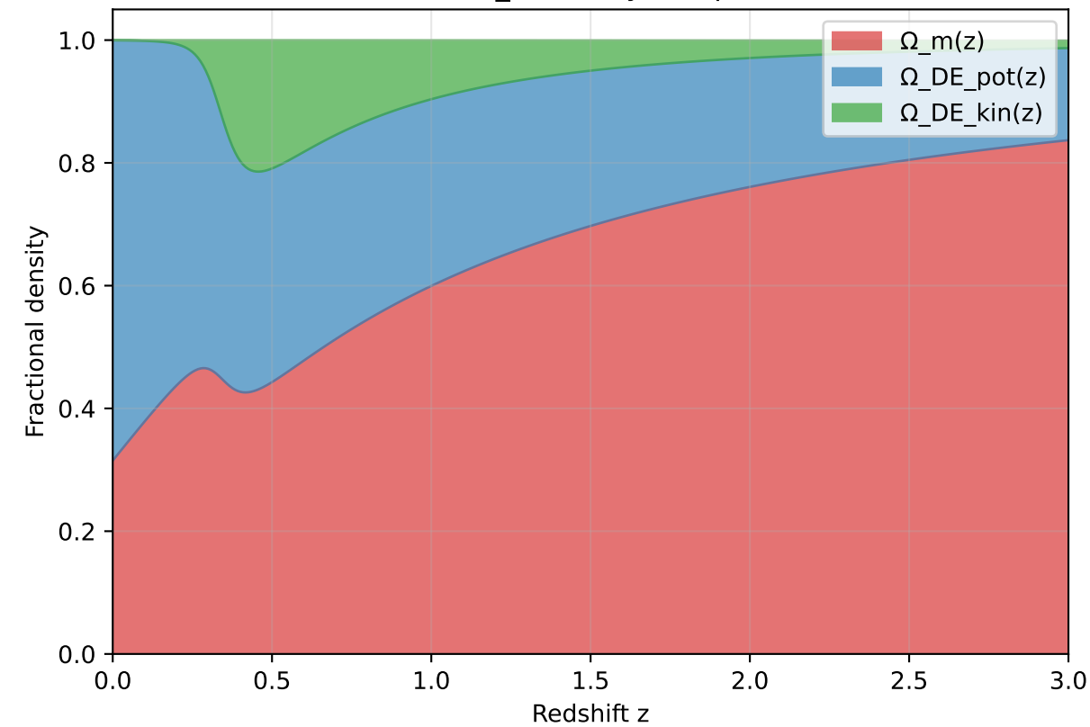
Model-A V_3 density components
