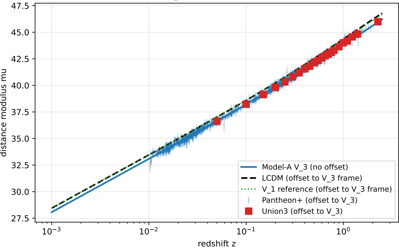
Hubble diagram (Pantheon+ + Union3)
