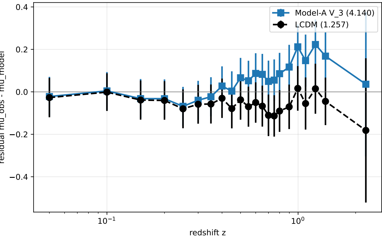
Union3 residuals
