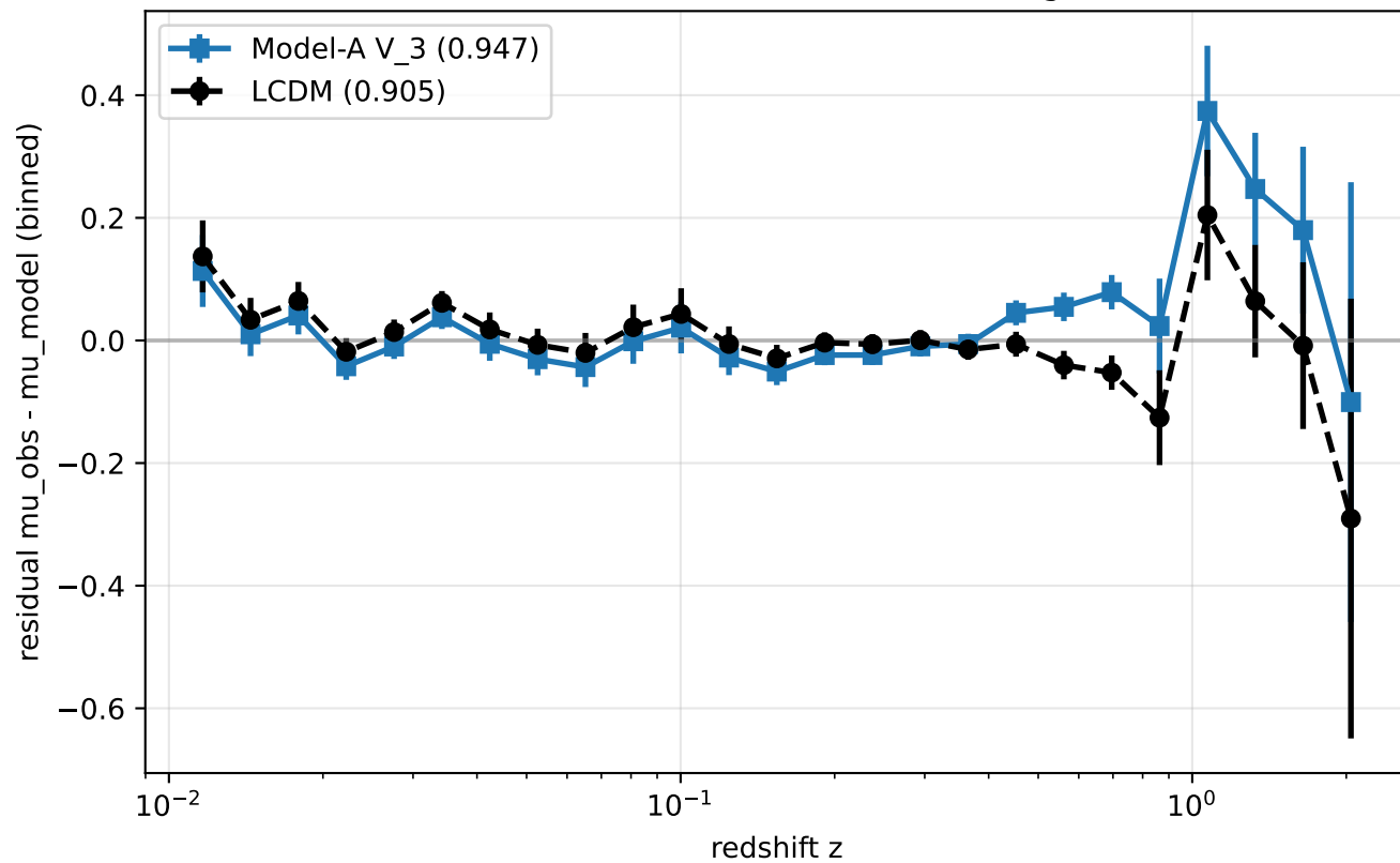
Pantheon+ residuals ( \chi^2/\text{dof} in legend)
