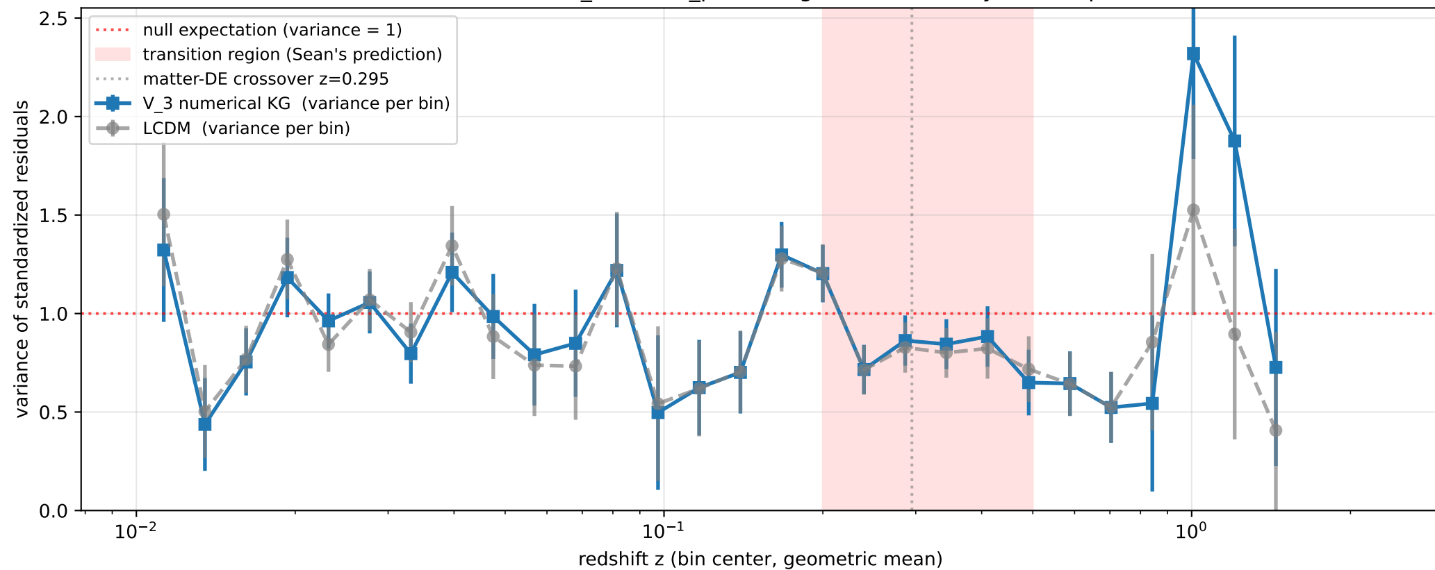
Per-bin variance of (\mu_{\text{obs}} - \mu_{\text{pred}}) / \sigma — continuity-scatter prediction
