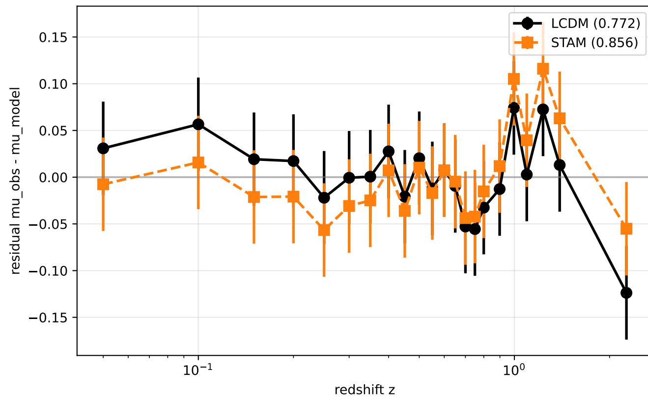
Union3 residuals
