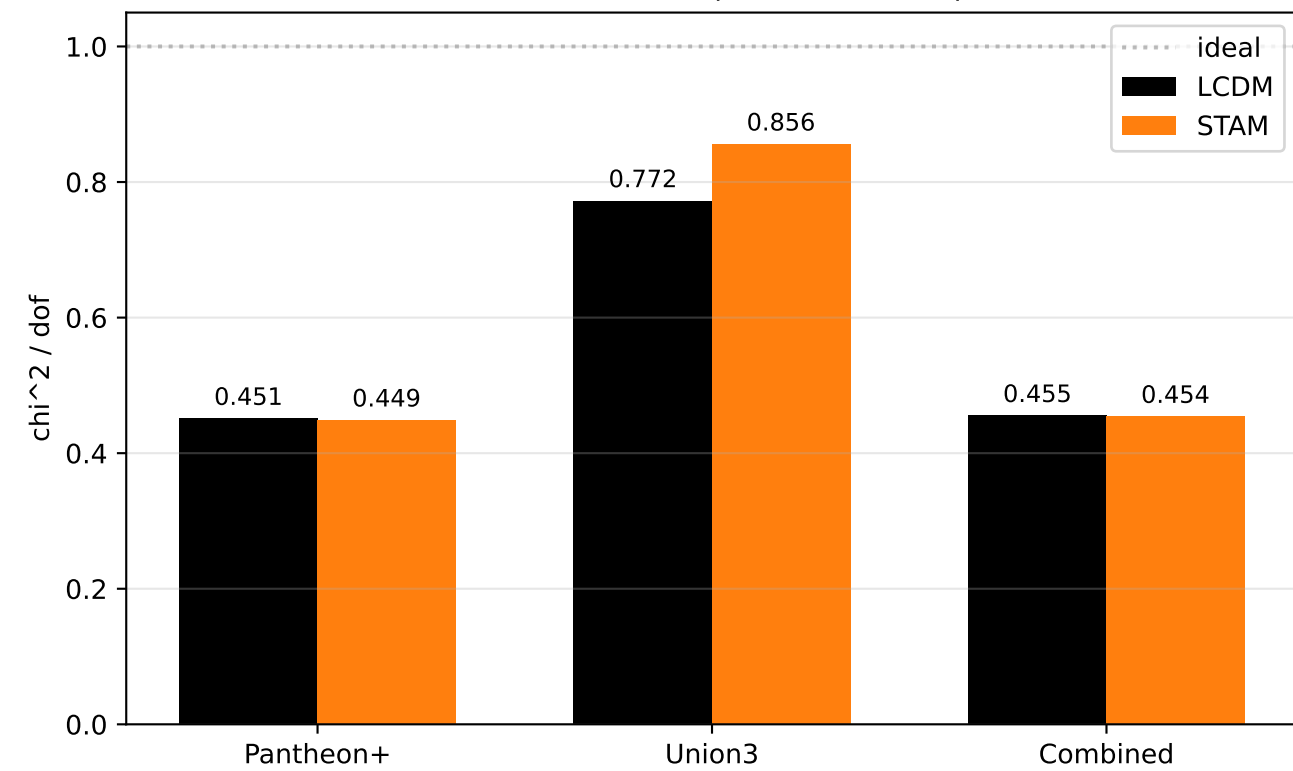
Goodness of fit (lower is better)
