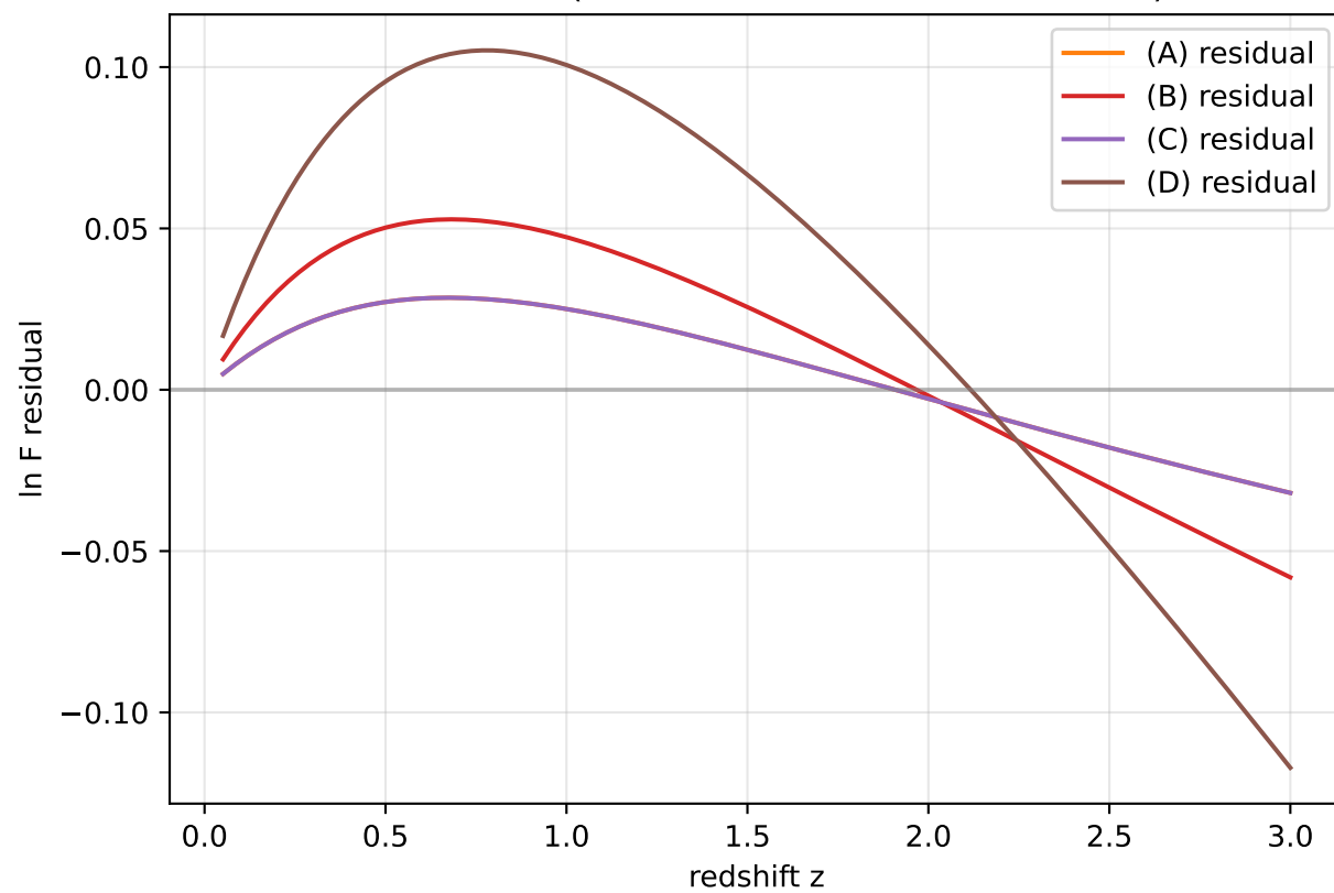
Fit residuals (smaller = better functional form)
