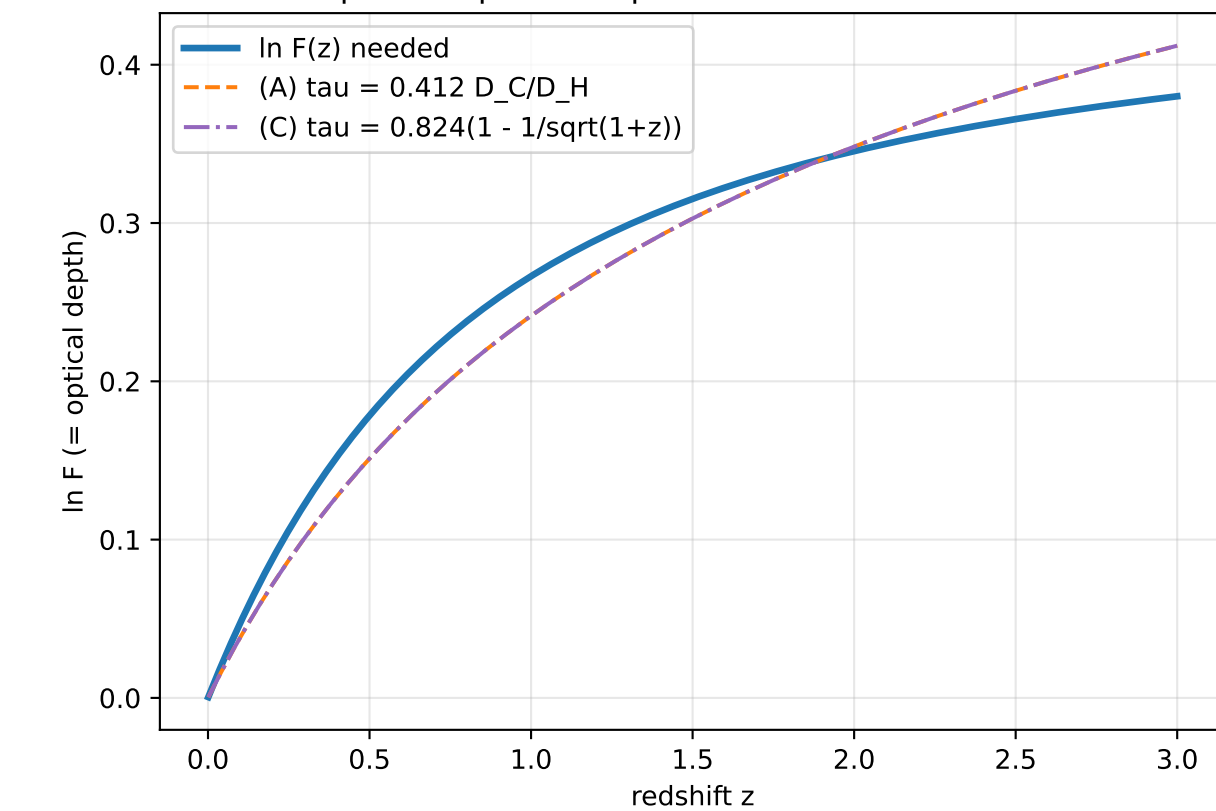
"Optical depth" interpretation of STAM correction
