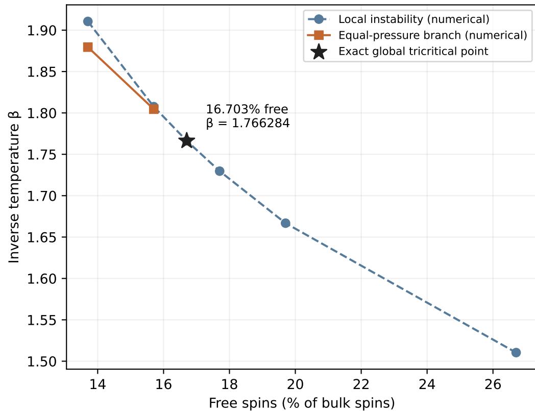
Chain construction · \kappa = 0.155498
