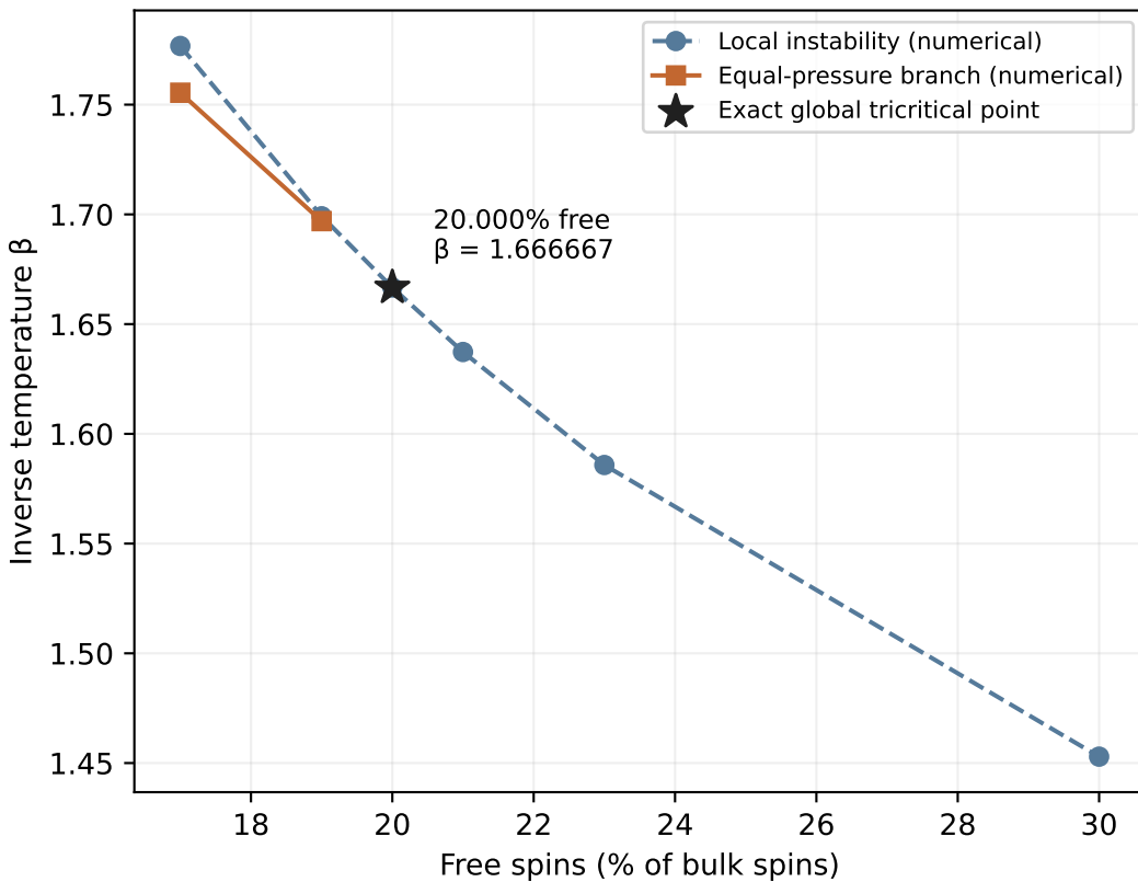
Pair construction · \kappa = 0.164792
