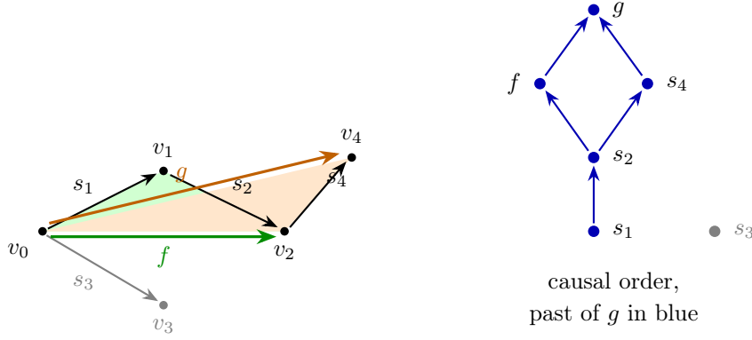
Figure 4: Example 3.7 drawn out. Left: the simplicial set after the six events, with the composite edges supplied by the fills f (green) and g (orange) and their witnessing 2-cells shaded to match. Right: the causal order as a Hasse diagram. The events f and s_4 are incomparable, which is what gives J^-(g) its two linearizations. The event s_3 and the vertex v_3 it created (grey) lie outside the causal past of g , so neither enters the state at g .
