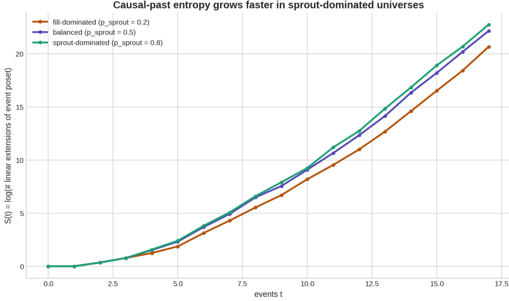
Figure 1: Causal-past entropy S(t) (mean over six seeds, 18 events) for three sprout probabilities. Entropy is monotone in every run and ordered by the sprout fraction at every time: sprouts create causally independent events (parallelism), fills create dependencies (sequentialization).
