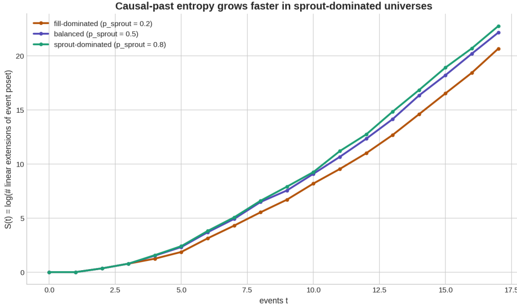
Figure 1: Causal-past entropy S(t) (mean over six seeds, 18 events) for three sprout probabilities. Entropy is monotone in every run and ordered by the sprout fraction at every time: sprouts create causally independent events (parallelism), fills create dependencies (sequentialization).
