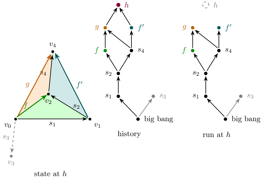
Figure 4: Example 3.12. Left: the state at h , the simplicial set itself, with sprout edges plain and the three composites colored by the fill that supplied them; the face (v_0, v_1, v_4) (purple) and the solid tetrahedron come from h . Middle: the history, with h (purple) a dimension-three fill sitting above the fills it depends on. Right: the run at h , the same order with h forgotten, since h adds no edge. The history remembers every event, the run drops the higher fill, and the state drops the order and the labels.
