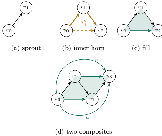
Figure 3: The two moves and what each of them adds. In (a) a vertex sprouts a fresh directed edge to a new vertex. After a second sprout, (b) shows the composable pair v_0 \rightarrow v_1 \rightarrow v_2 whose composite is absent, an unfilled inner horn \Lambda_1^2 (amber, missing edge dashed). In (c) the fill supplies the composite v_0 \rightarrow v_2 (green) together with the 2-simplex witnessing it (shaded). Panel (d) shows the state after a third sprout and both first-tier fills. Two distinct horns now call for a composite from v_0 to v_3 , one built from v_0 \rightarrow v_1 with v_1 \rightarrow v_3 and one from v_0 \rightarrow v_2 with v_2 \rightarrow v_3 . Each fill mints its own composite, so a and b are parallel edges rather than a single shared one. Only once both are present does the inner horn \Lambda_1^3 exist, since its three faces already carry all six edges of \Delta^3 ; filling it therefore adds a 2-simplex and a 3-simplex but no edge. Only inner horns are ever filled, so edge direction is never inverted and the limit object is a quasicategory.
