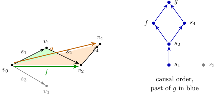
Figure 4: Example 3.8. Left: the simplicial set after the six events, with the composite edges supplied by the fills f (green) and g (orange) and their witnessing 2-cells shaded to match. Right: the causal order as a Hasse diagram. The events f and s_4 are incomparable, which is what gives J^-(g) its two linearizations. The event s_3 and the vertex v_3 it created (grey) lie outside the causal past of g , so neither enters the state at g .
