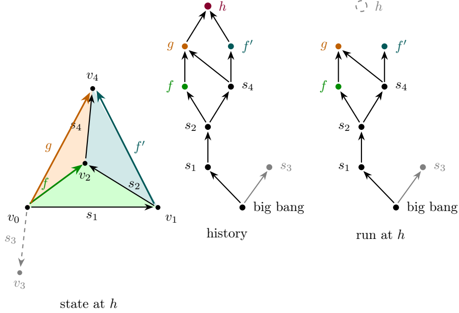
Figure 4: Example 3.9. Left: the state at h , the simplicial set itself, with sprout edges plain and the three composites colored by the fill that supplied them; the face (v_0, v_1, v_4) (purple) and the solid tetrahedron come from h . Middle: the history, with h (purple) a dimension-three fill sitting above the fills it depends on. Right: the run at h , the same order with h forgotten, since h adds no edge. The history remembers every event, the run drops the higher fill, and the state drops the order and the labels.
