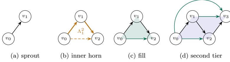
Figure 3: Two moves generate the growth. In (a) a vertex sprouts a fresh directed edge. After a second sprout, (b) shows the composable pair v_0 \rightarrow v_1 \rightarrow v_2 whose composite is absent, an unfilled inner horn \Lambda_1^2 (amber, missing edge dashed). In (c) the fill supplies the composite v_0 \rightarrow v_2 (green) together with the 2-cell witnessing it (shaded). Panel (d) shows the state after one further sprout and fill at the first tier, followed by a fill at the second: the two routes v_0 \rightarrow v_2 \rightarrow v_3 and v_0 \rightarrow v_1 \rightarrow v_3 both demand the edge v_0 \rightarrow v_3 , and a single 3-cell (shaded, drawn as the quadrilateral v_0v_1v_3v_2 ) makes them agree. Only inner horns are ever filled, so edge direction is never inverted and the limit object is a quasicategory.
