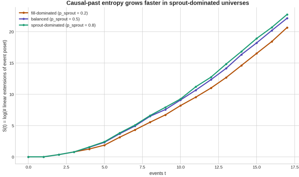
Figure 2: Causal-past entropy S(t) (mean over six seeds, 18 events) for three sprout probabilities. Entropy is monotone in every run and ordered by the sprout fraction at every time: sprouts create causally independent events (parallelism), fills create dependencies (sequentialization).
