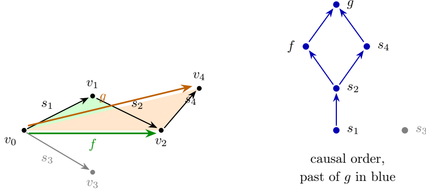
Figure 4: Example 3.7. Left: the simplicial set after the six events, with the composite edges supplied by the fills f (green) and g (orange) and their witnessing 2-cells shaded to match. Right: the causal order as a Hasse diagram. The events f and s_4 are incomparable, which is what gives J^-(g) its two linearizations. The event s_3 and the vertex v_3 it created (grey) lie outside the causal past of g , so neither enters the state at g .
