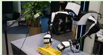
Two eggs→box
