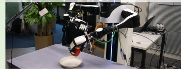
Apple→plate
