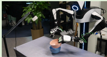
Bowl→bowl
