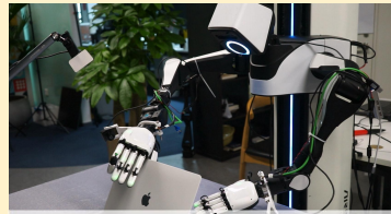
Open laptop
