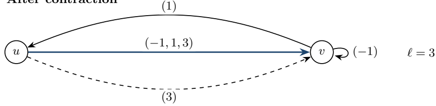
FIGURE 5. An exact contraction. The vertex x has one outgoing edge; u and v are macro vertices because each has two outgoing edges. The words (-1) and (1, 3) concatenate to (-1, 1, 3) , whose length remains three. All other edges are retained. Line styles identify corresponding edges.
