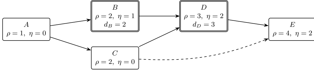
Illustrative condensation DAG (not the full computed graph)
