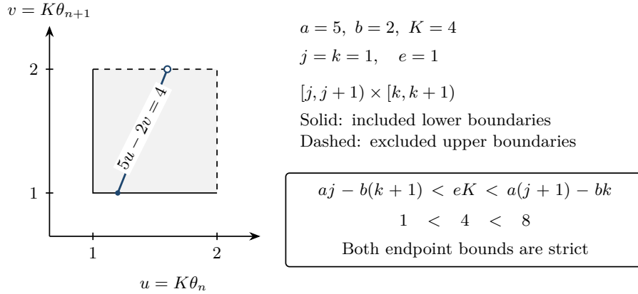
FIGURE 2. Cell compatibility for a = 5, b = 2, K = 4, j = k = 1, e = 1 . The line meets the half-open square along u = (4 + 2v)/5 , 1 \leq v < 2 . The lower endpoint is included and the upper endpoint is excluded. The cell-pair test is local; it does not assert the existence of a full orbit.
