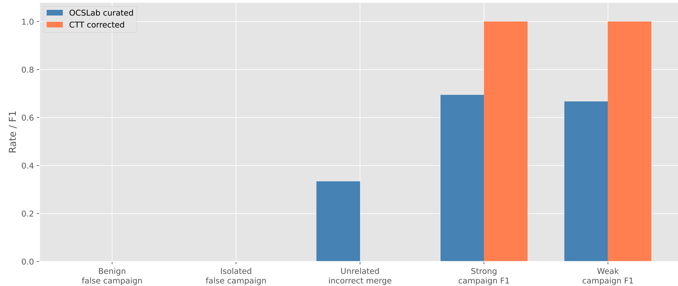
Fleet-correlation outcomes: OCSLab vs corrected CTT (200-node graphs)
