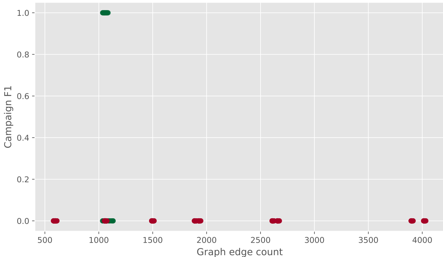
Campaign F1 vs graph edge count
