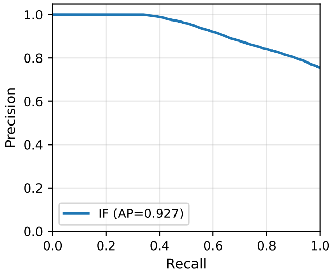
Precision-Recall — Local IDS (Test)
