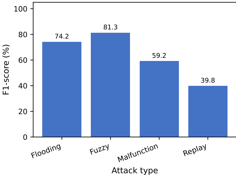
Local IDS F1-score by Attack Type (Test)
