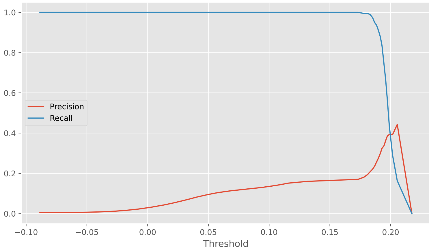
Precision-recall vs threshold
