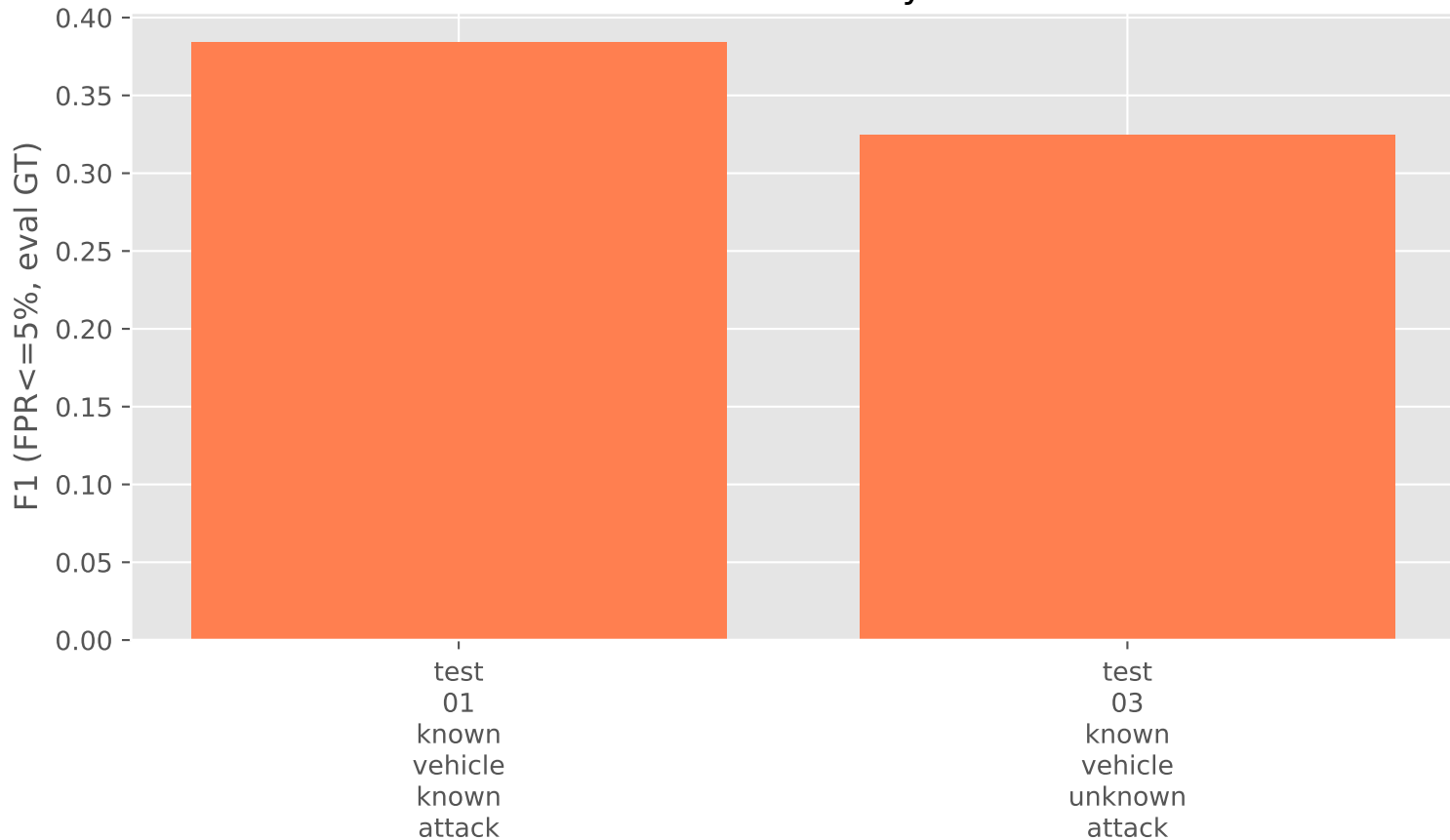
Corrected local F1 by subset
