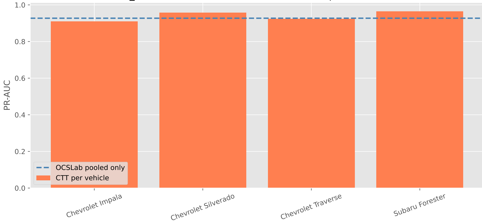
LOCAL_COMP2 — Per-vehicle PR-AUC (OCSLab pooled reference)
